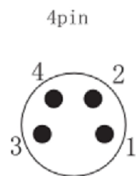
Pin assignment front view/针位分布前视图
